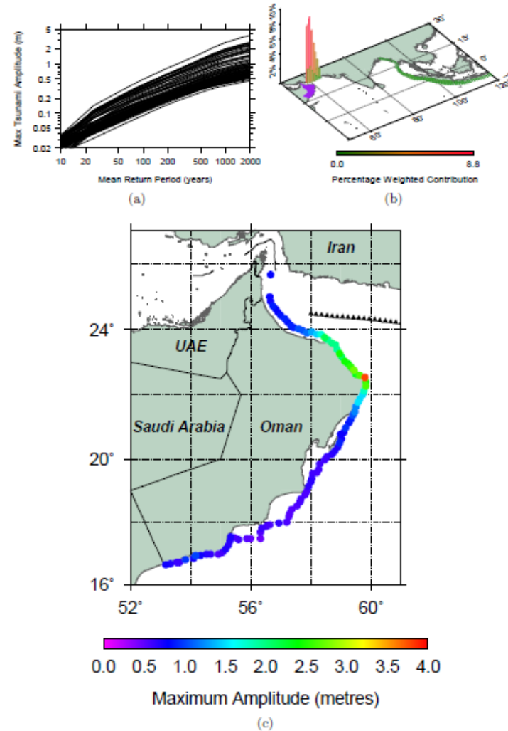
Figure 43: Oman:- (a) Hazard curves for all model output points. (b) National weighted deaggregated hazard. (c) Maximum amplitude at a 2000 year return period for all model output points.
