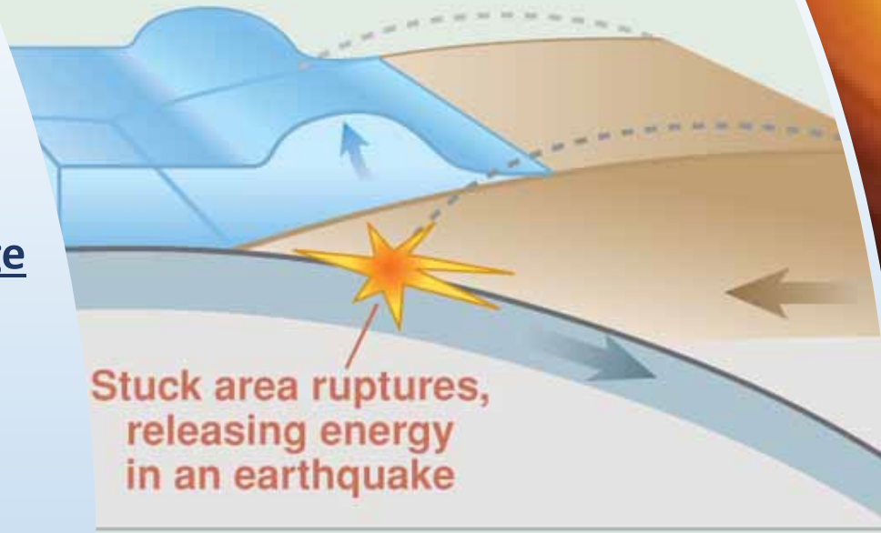
Earthquake starts tsunami
