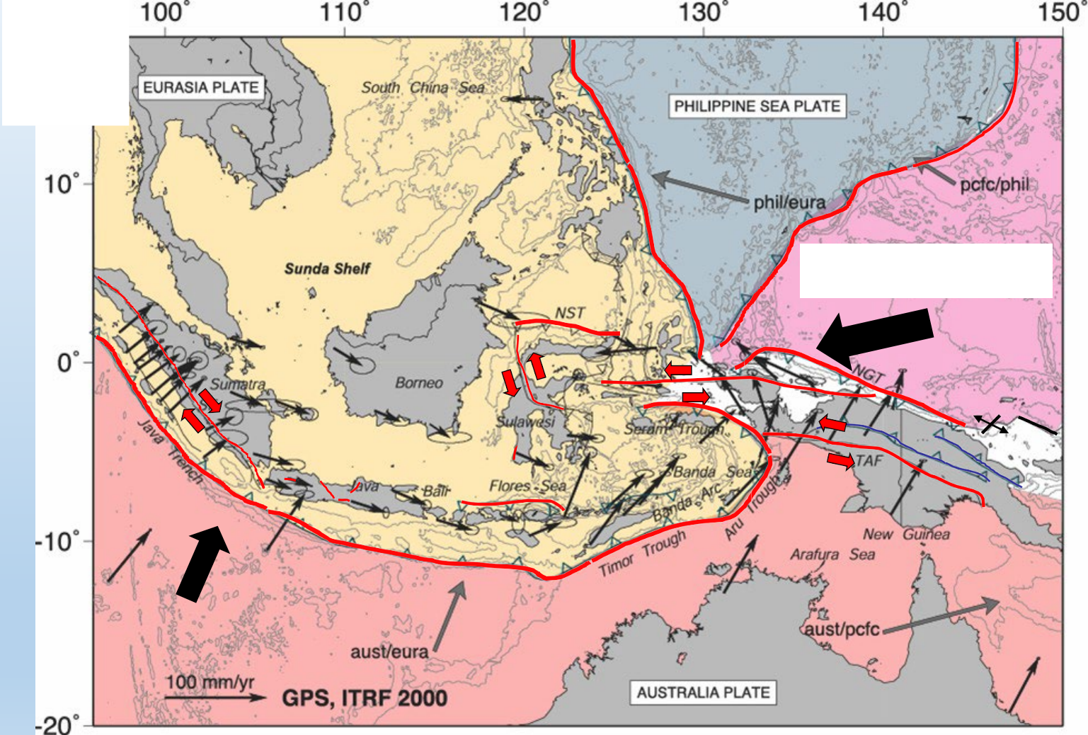
ACTIVE TECTONICS of INDONESIA
