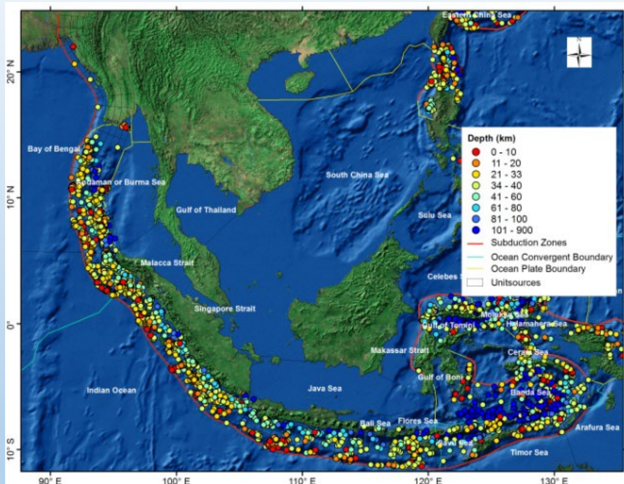
Historical database (HARVARD)
