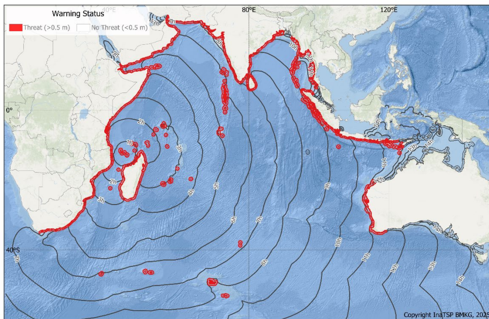
Figure S3-32. Bulletin 10: Tsunami Threat Map to the 12-hour isochrone (travel time contour).
