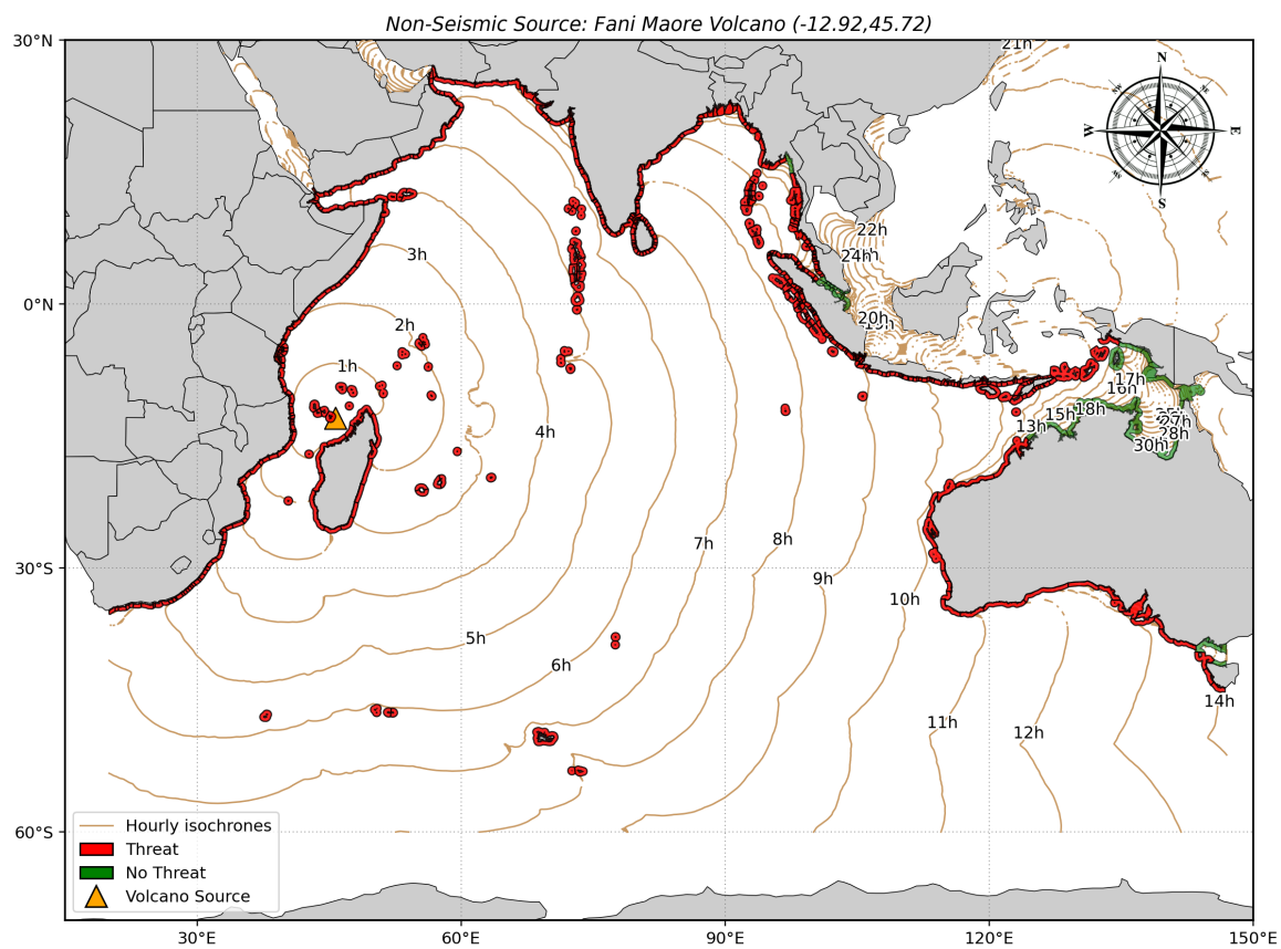
Figure S3-21. Bulletin 12: Tsunami Threat Map to the 14-hour isochrone (travel time contour).
