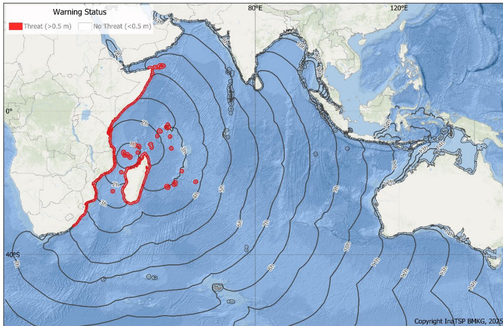
Figure S3-25. Bulletin 3: Tsunami Threat Map to the 5-hour isochrone (travel time contour).
