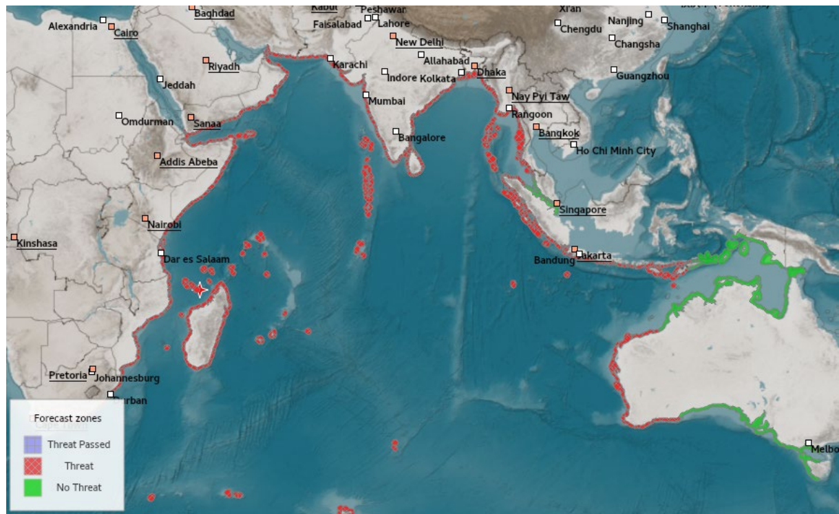
Figure S3-09. Bulletin 8-12: Tsunami Threat Map to the 12-hour isochrone (travel time contour).
