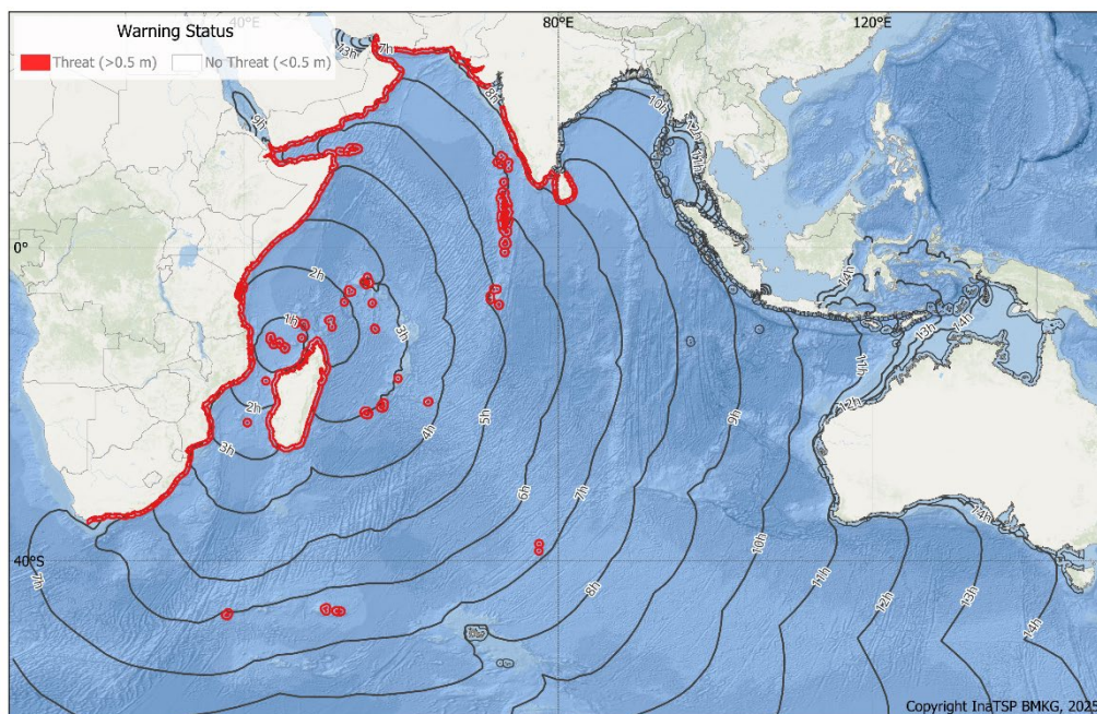
Figure S3-28. Bulletin 6: Tsunami Threat Map to the 8-hour isochrone (travel time contour).
