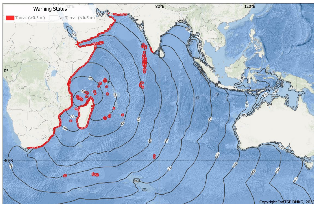
Figure S3-27. Bulletin 5: Tsunami Threat Map to the 7-hour isochrone (travel time contour).
