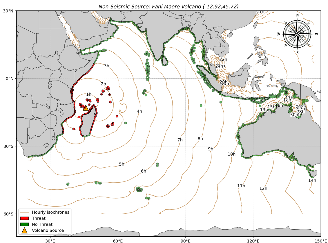
Figure S3-10. Bulletin 1: Tsunami Threat Map to the 3-hour isochrone (travel time contour).
