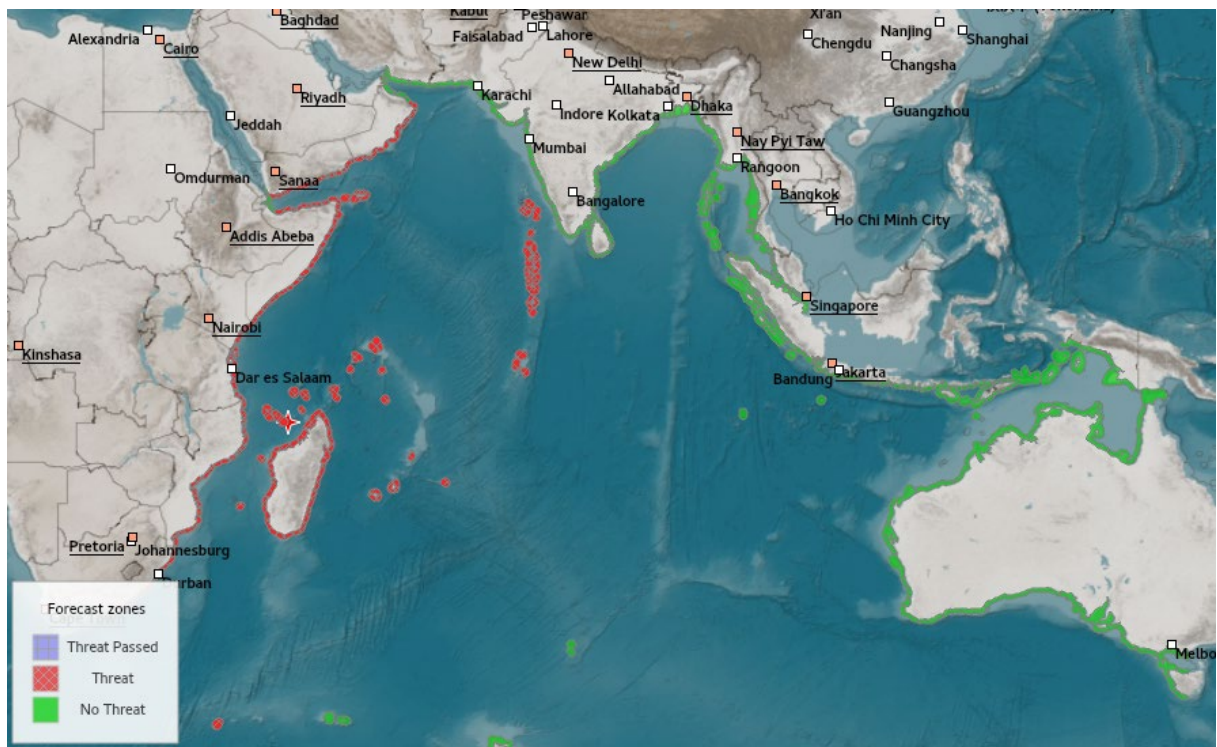
Figure S3-03. Bulletin 2: Tsunami Threat Map to the 6-hour isochrone (travel time contour).
