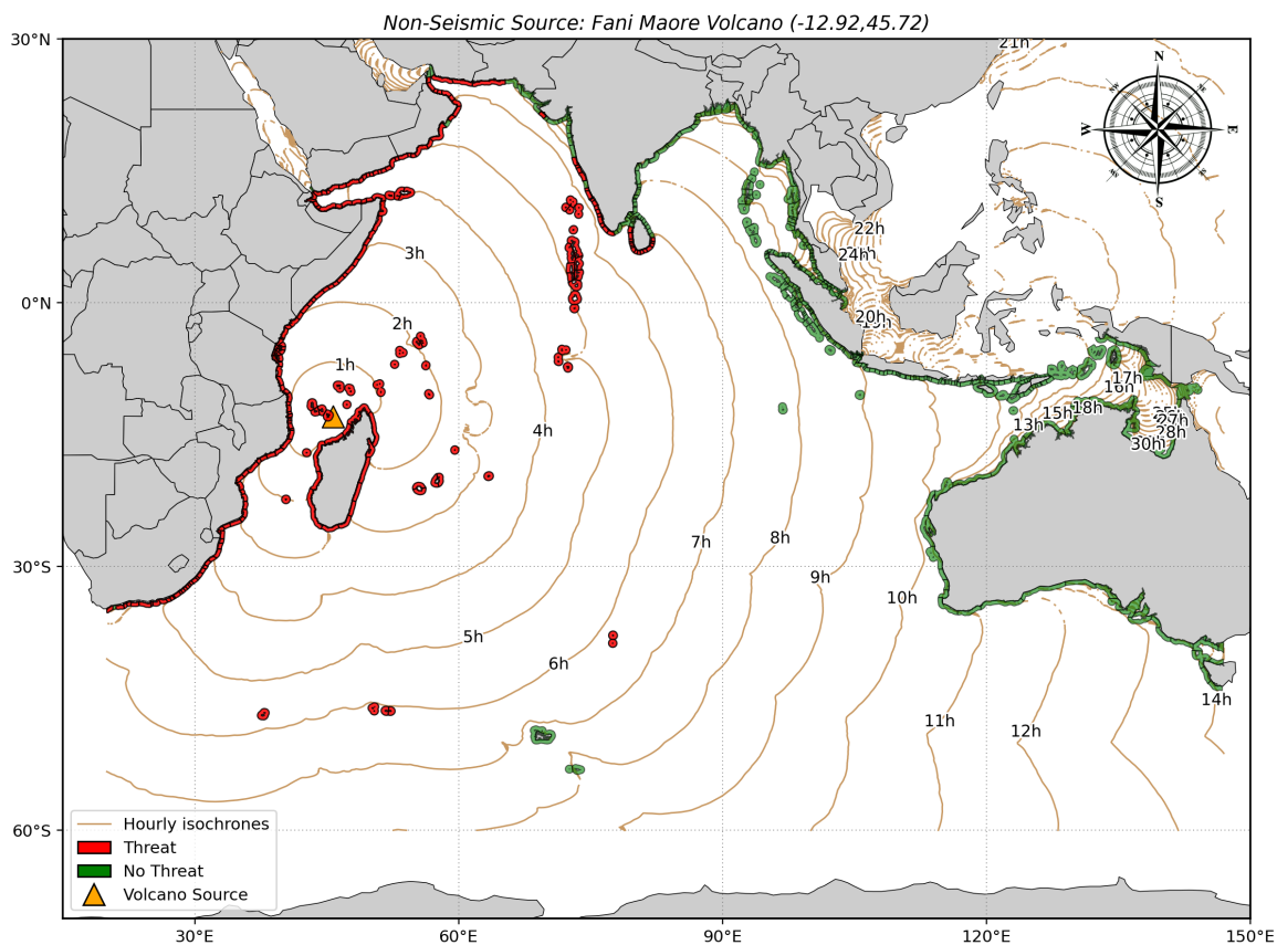
Figure S3-14. Bulletin 5: Tsunami Threat Map to the 7-hour isochrone (travel time contour).
