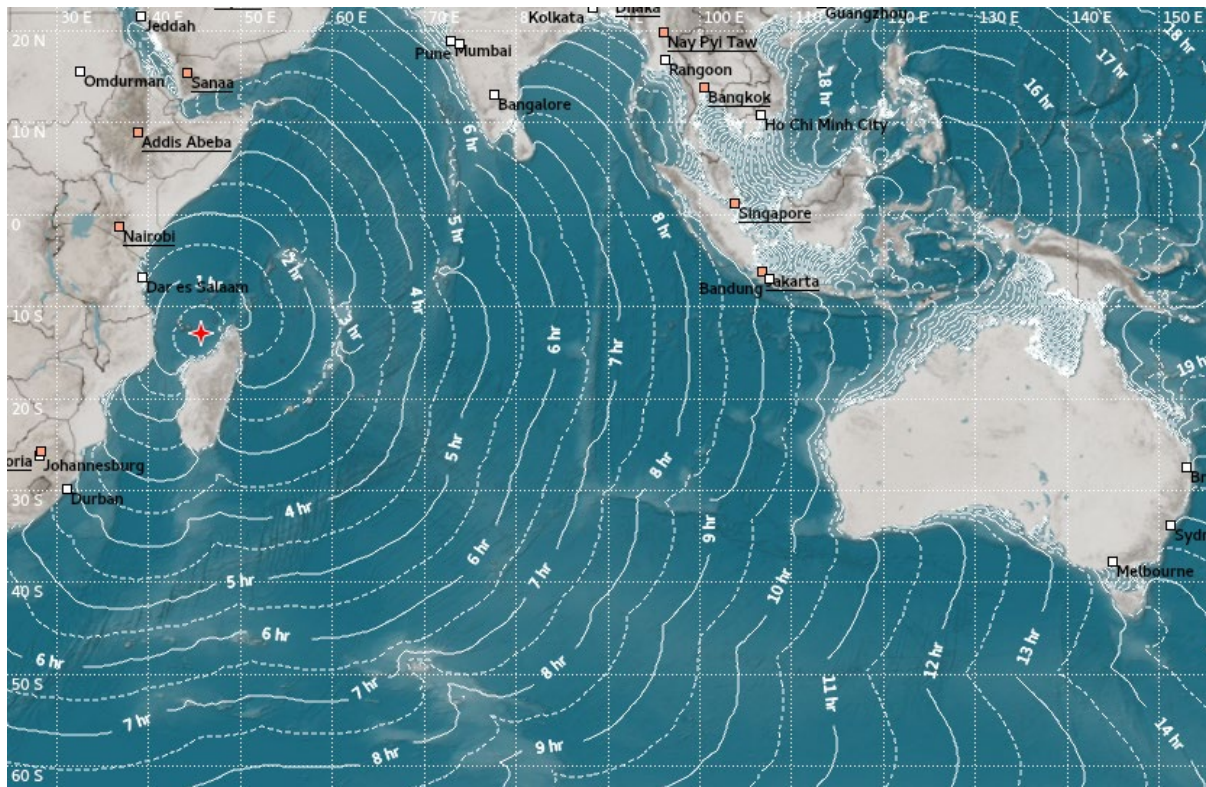
Figure S3-01. Travel Time Map
