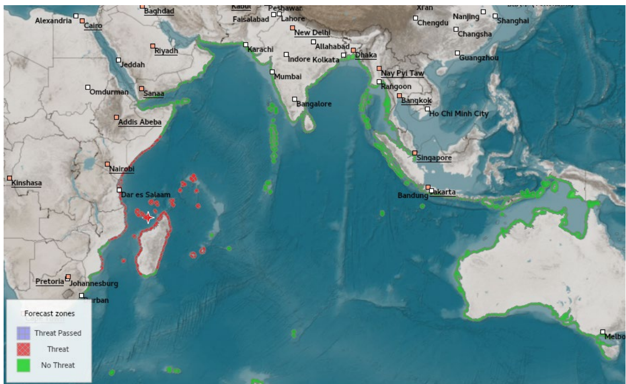
Figure S3-02. Bulletin 1: Tsunami Threat Map to the 3-hour isochrone (travel time contour).
