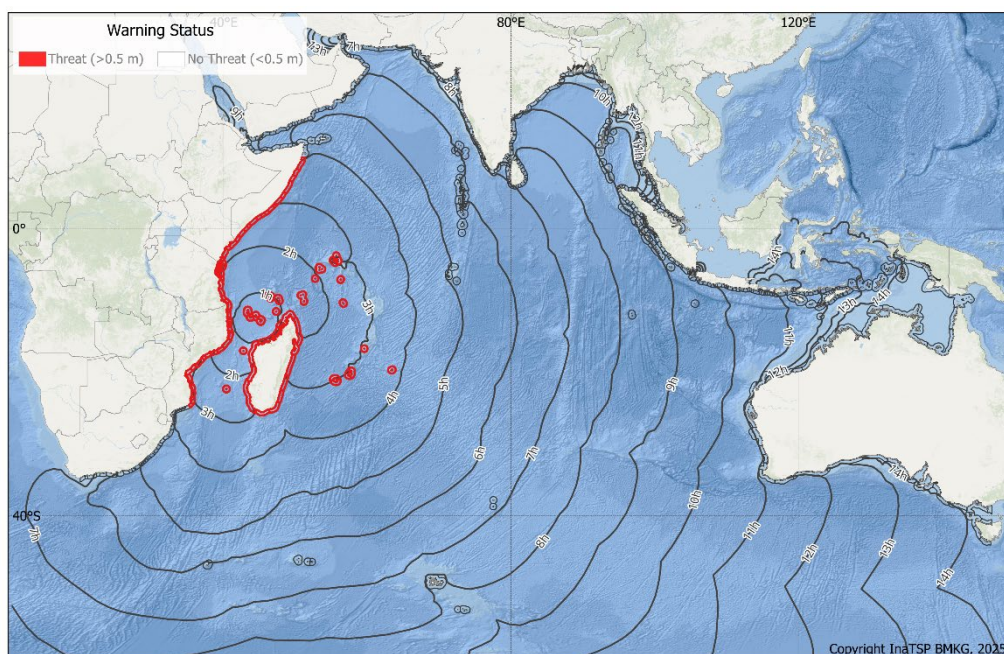
Figure S3-24. Bulletin 2: Tsunami Threat Map to the 4-hour isochrone (travel time contour).
