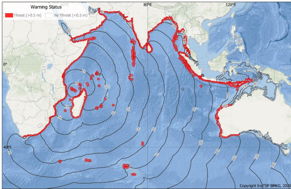
Figure S3-33. Bulletin 11: Tsunami Threat Map to the 13-hour isochrone (travel time contour).
