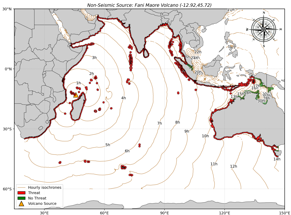
Figure S3-22. Bulletin 13: Tsunami Threat Map to the 15-hour isochrone (travel time contour).
