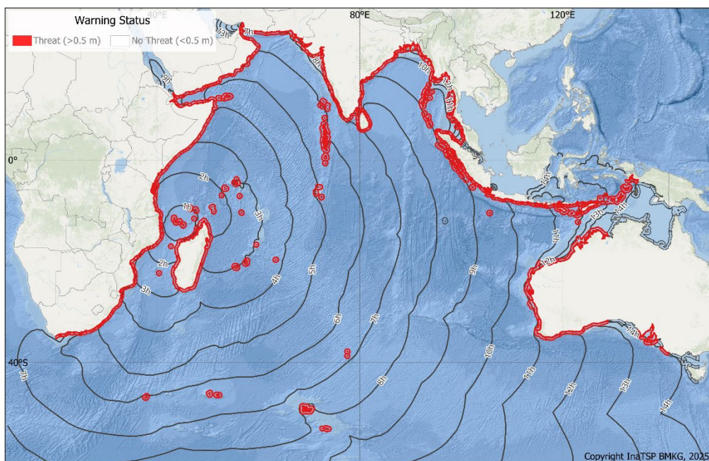
Figure S3-29. Bulletin 12: Tsunami Threat Map to the 14-hour isochrone (travel time contour).
