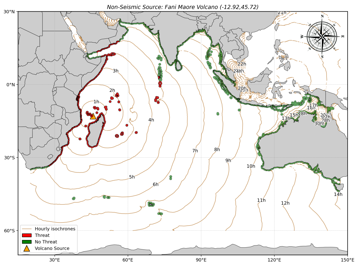
Figure S3-12. Bulletin 3: Tsunami Threat Map to the 5-hour isochrone (travel time contour).
