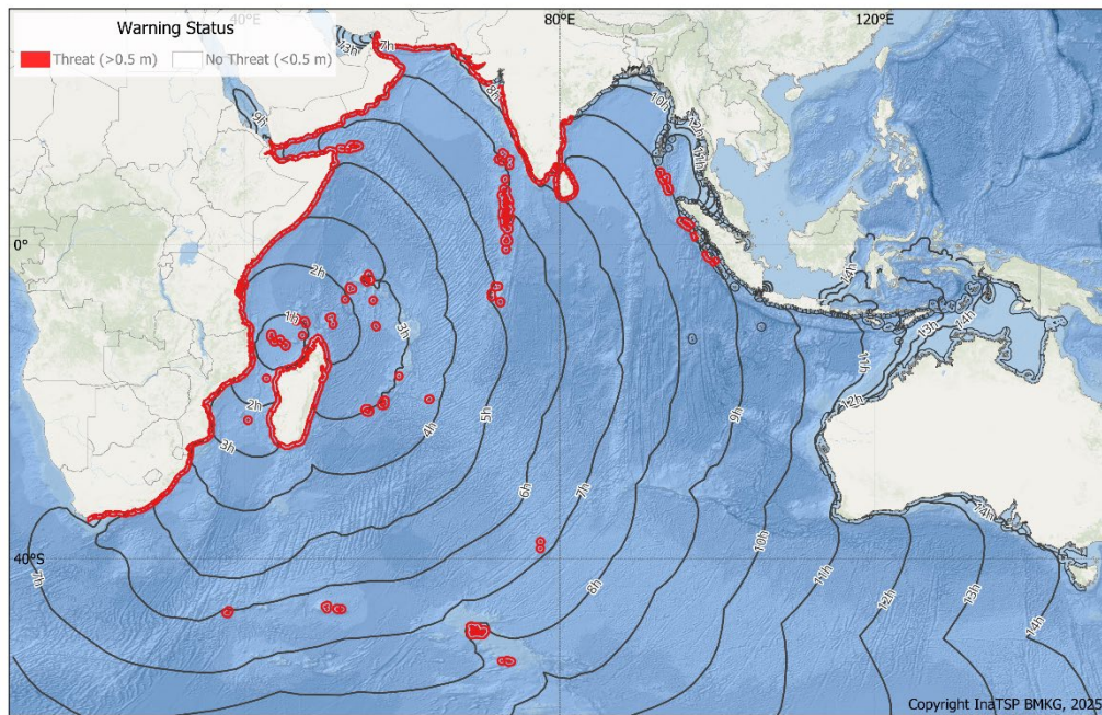
Figure S3-29. Bulletin 7: Tsunami Threat Map to the 9-hour isochrone (travel time contour).
