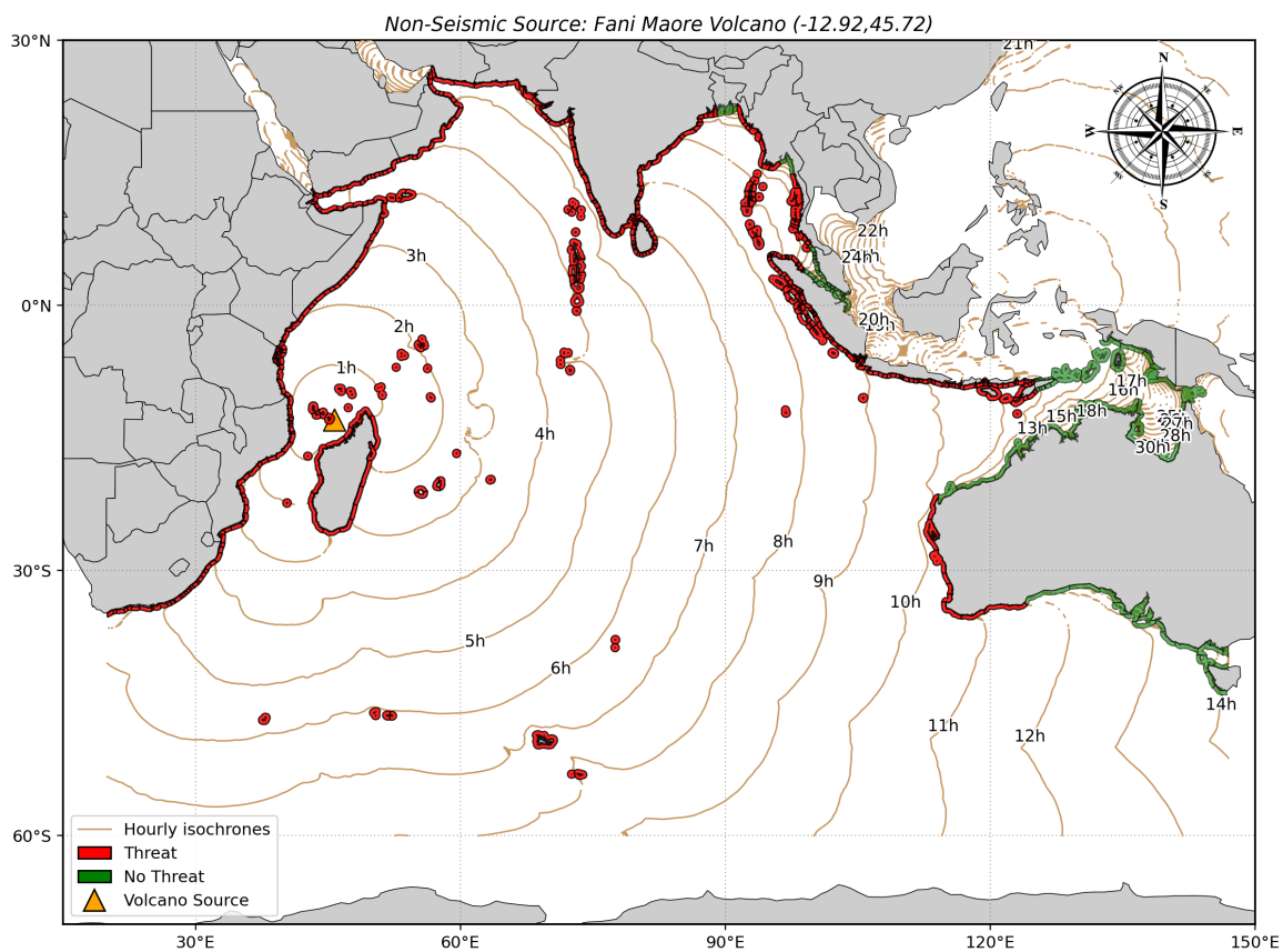
Figure S3-19. Bulletin 10: Tsunami Threat Map to the 12-hour isochrone (travel time contour).
