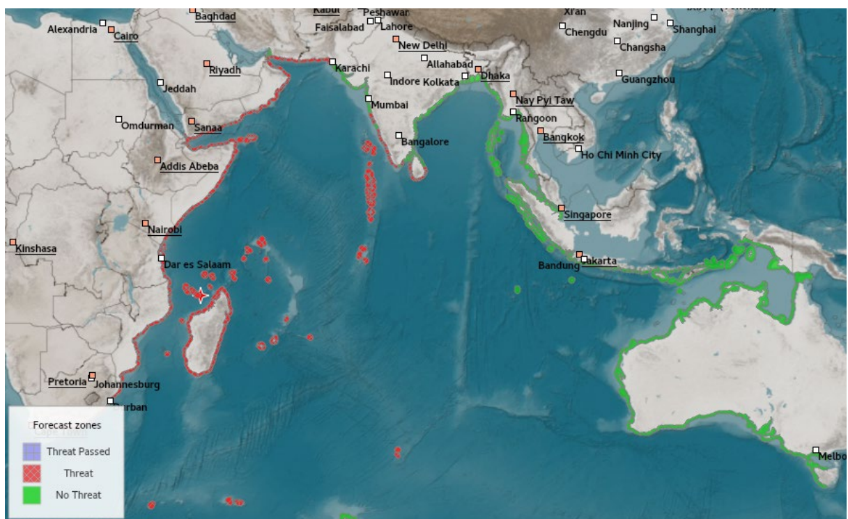
Figure S3-04. Bulletin 3: Tsunami Threat Map to the 7-hour isochrone (travel time contour).
