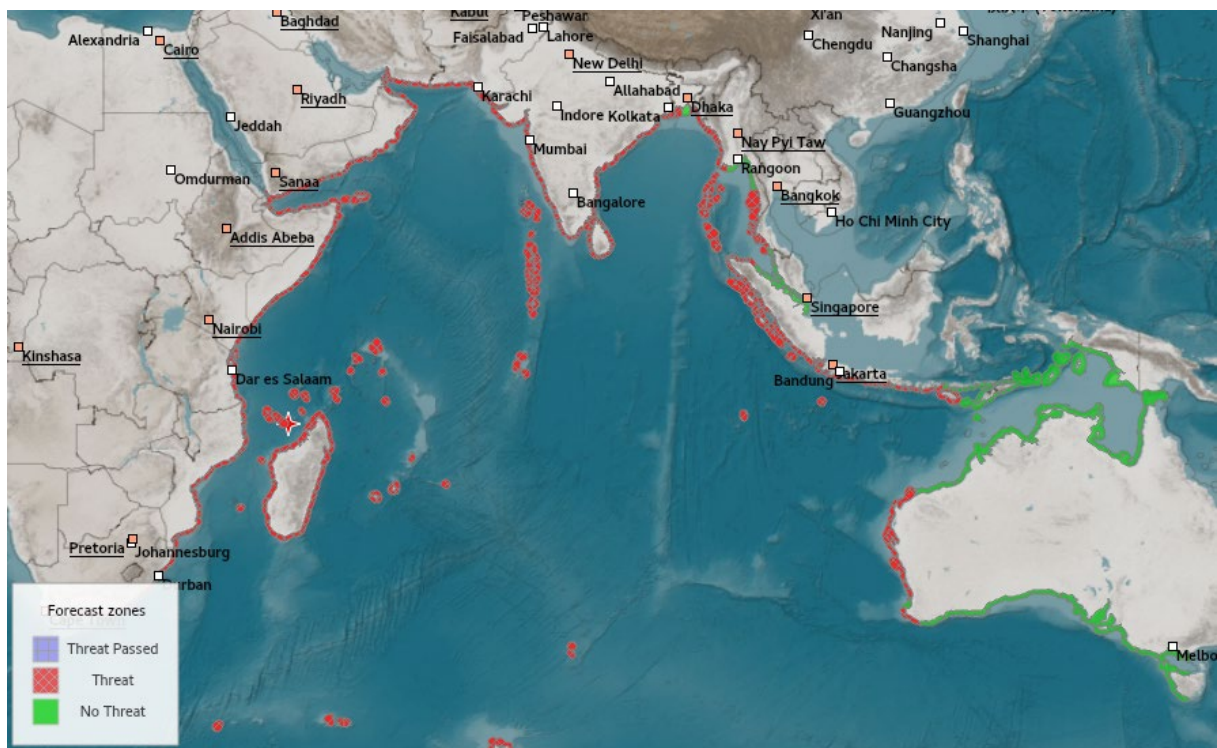
Figure S3-08. Bulletin 7: Tsunami Threat Map to the 11-hour isochrone (travel time contour).
