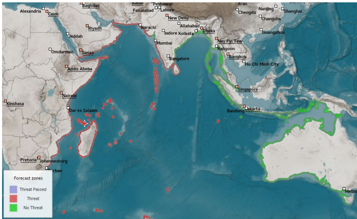
Figure S3-05. Bulletin 4: Tsunami Threat Map to the 8-hour isochrone (travel time contour).
