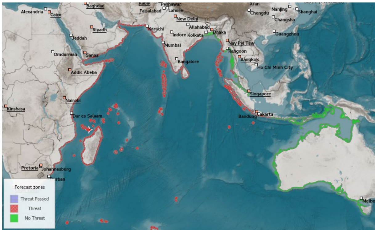
Figure S3-07. Bulletin 6: Tsunami Threat Map to the 10-hour isochrone (travel time contour).
