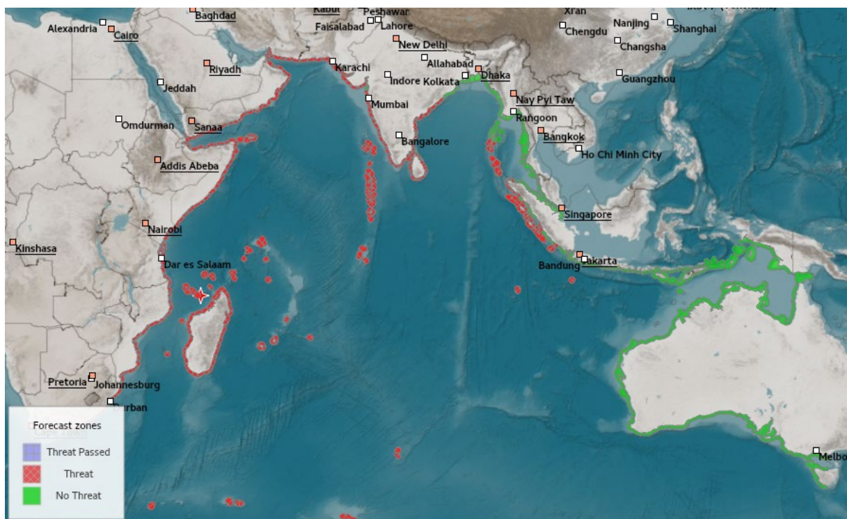
Figure S3-06. Bulletin 5: Tsunami Threat Map to the 9-hour isochrone (travel time contour).
