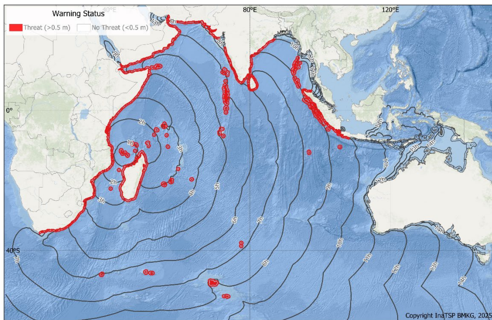
Figure S3-30. Bulletin 8: Tsunami Threat Map to the 10-hour isochrone (travel time contour).
