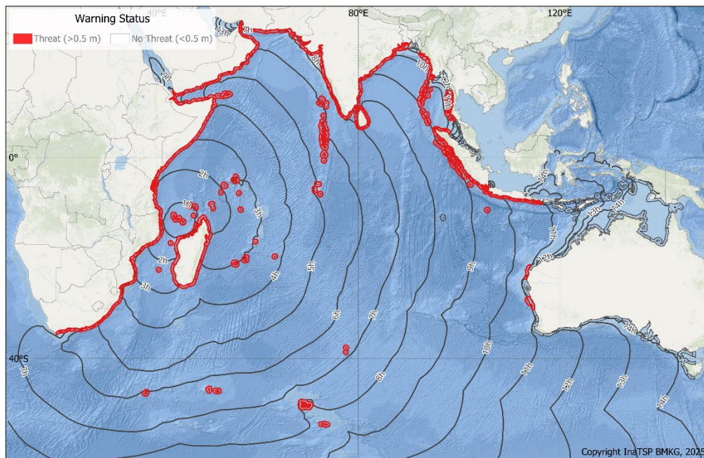
Figure S3-31. Bulletin 9: Tsunami Threat Map to the 11-hour isochrone (travel time contour).
