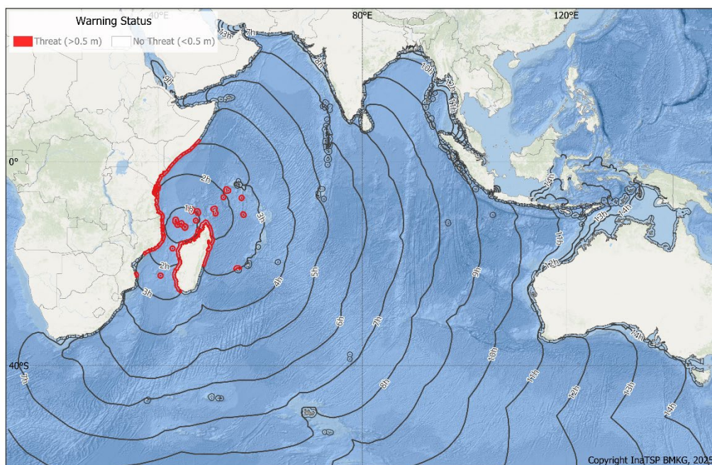
Figure S3-23. Bulletin 1: Tsunami Threat Map to the 3-hour isochrone (travel time contour).
