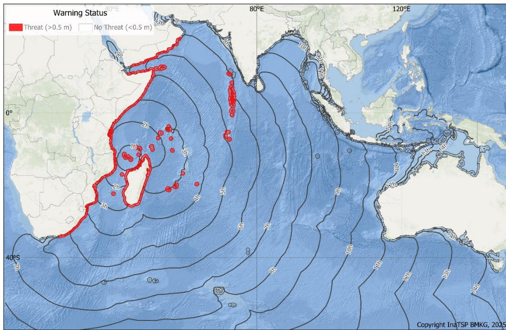
Figure S3-26. Bulletin 4: Tsunami Threat Map to the 6-hour isochrone (travel time contour).
