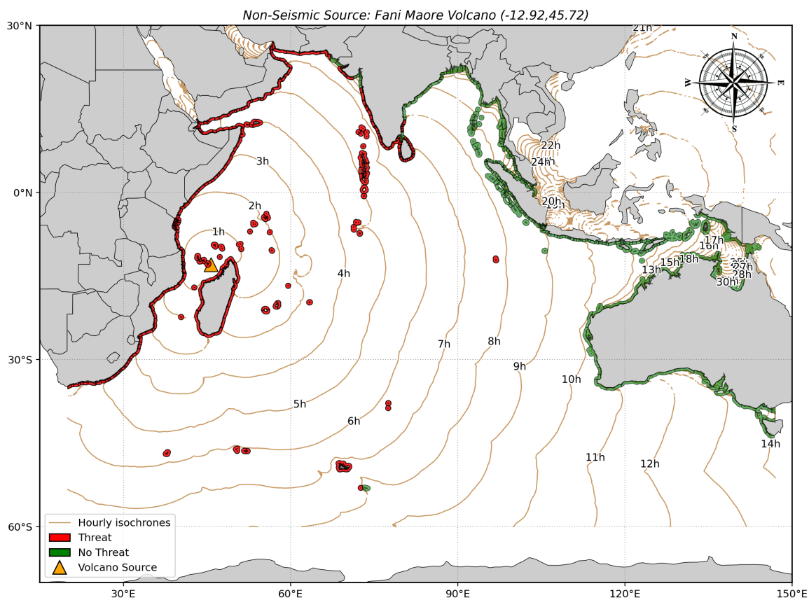
Figure S3-15. Bulletin 6: Tsunami Threat Map to the 8-hour isochrone (travel time contour).
