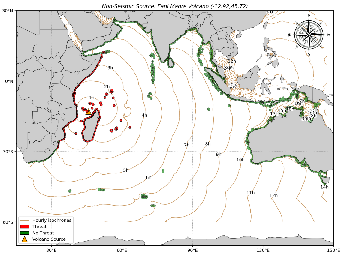
Figure S3-11. Bulletin 2: Tsunami Threat Map to the 4-hour isochrone (travel time contour).
