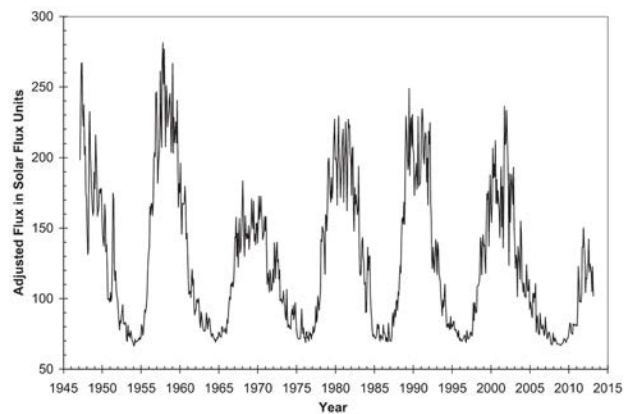
Figure 3. Radio observatory in Penticton, Canada (left) and its long-term observation of solar radio signal at 10.7 cm wavelength (right), showing the 11-year solar cycles (from Tapping, K. 2013,[12])
