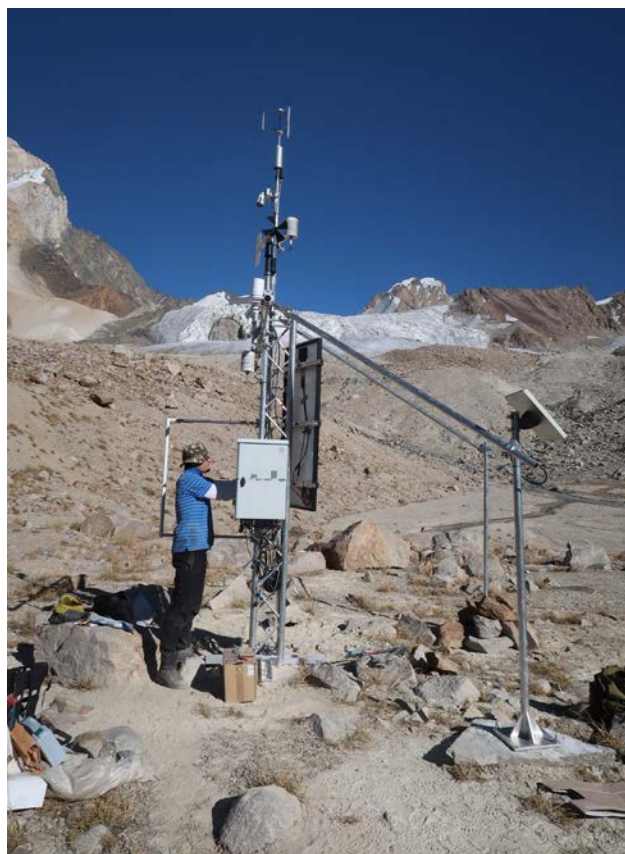
Figure 10. Sept 2021 installation of a new high mountain observation site in the Western Pamir, Tajikistan as part of the "Cryosphere Observations and Modelling for improved Adaptation in Central Asia" (CROMO-ADAPT) funded by the Swiss Development Corporation and co-led by University of Fribourg and WSL Institute of Snow and Avalanche Research SLF (Switzerland); photo Joel Fiddes (Switzerland).
