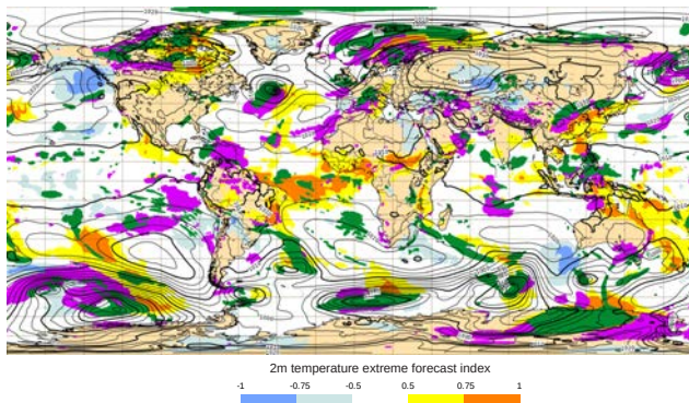
Figure 3. Extreme Forecast Index (EFI) map for 5 October 2021, showing where anomalous weather is likely to occur within the next seven days. The colours mark areas with likely high winds (magenta), heavy rainfall (green), high temperatures (yellow/orange) and low temperatures (light blue/blue). The EFI relies on climatologies and anomaly probabilities derived from reanalysis data. (Source: ECMWF)
