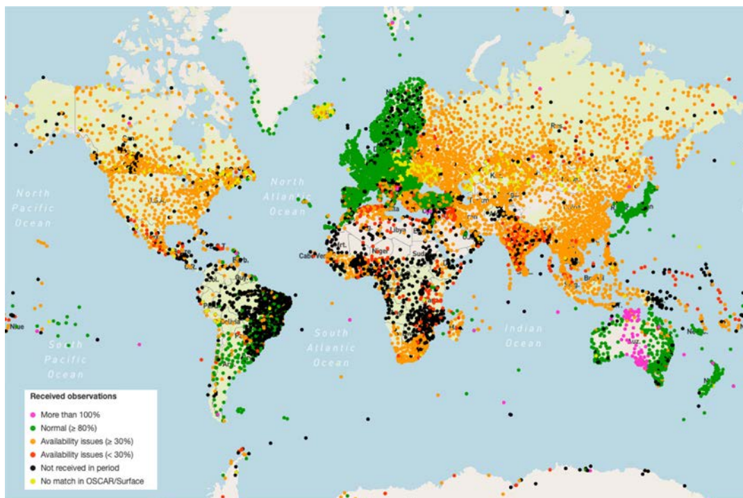
Figure 1. Surface pressure observations received by global NWP Centers on Sept 9 2021). (Source: WIGOS Data Quality Monitoring System)
