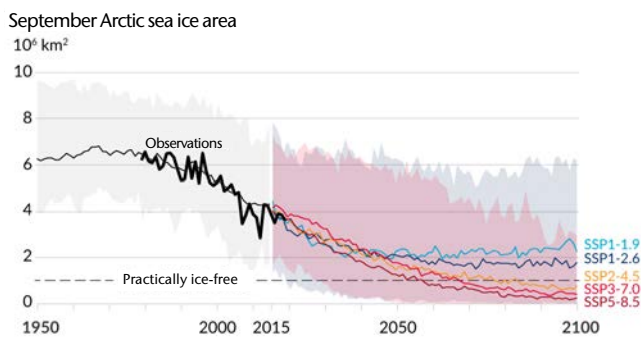
Figure 5. September Arctic sea ice area in 10^6 \text{ km}^2 based on satellite-based observations and CMIP6 model simulations. Very likely ranges are shown for SSP1-2.6 and SSP3-7.0. The Arctic is projected to be practically ice-free near mid-century under mid and high GHG emission scenarios. The figure is adapted from Figure SMP8 in IPCC (2021). Observations added by Prof Ed Hawkins ( http://www.climate-lab-book.ac.uk/2021/adding-observations/ ) – courtesy Thomas Lavergne (Norway).
