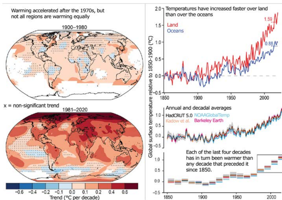
Figure 1. Subset of Figure 2.11 from IPCC AR6 WG1 showing trends and timeseries for global mean surface temperature reconstructed from land and marine meteorological observations. The HadCRUTv5 product includes substantial interpolation over data void regions. Source: IPCC AR6 Figure 2.11
