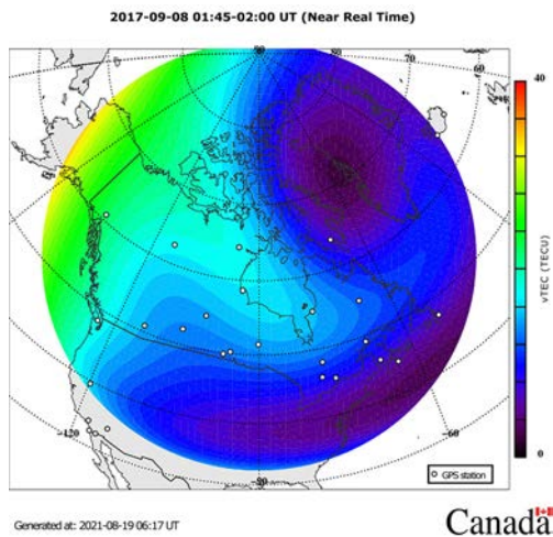
Figure 7. Left: Map of Total Electron Content of the ionosphere over Canada obtained using GNSS data ( https://www.spaceweather.gc.ca/data-donnee/ionosphere/index-en.php ). Right: Map of GNSS tracking stations ( https://igs.org/network/ ).
